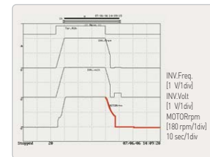
▶ DC braking
